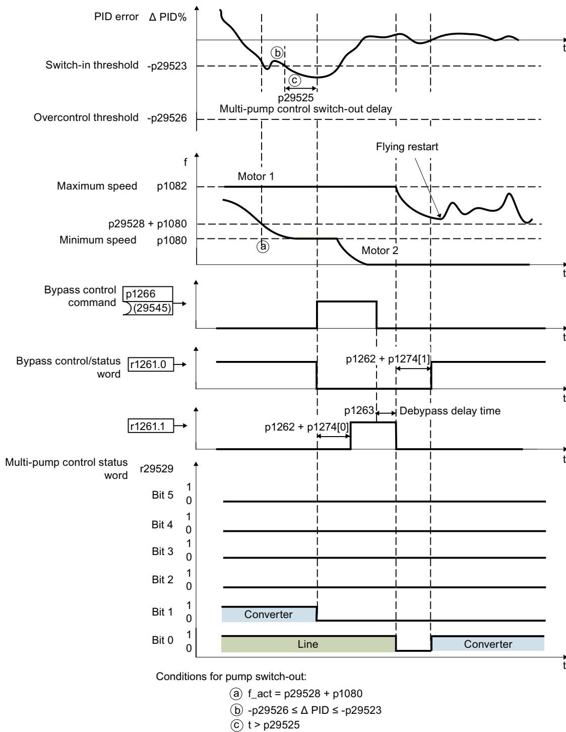
Figure 6-33 Pump switch-out based on the fixed sequence (p29522 = 0)
