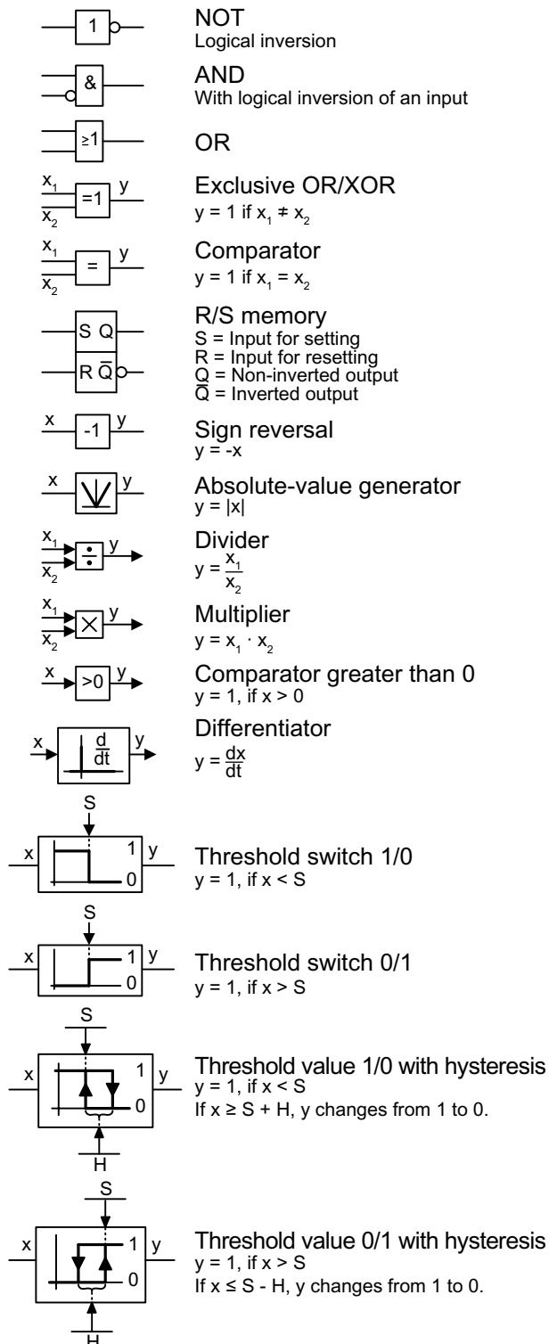
Figure 6-110 Binary and analog blocks
