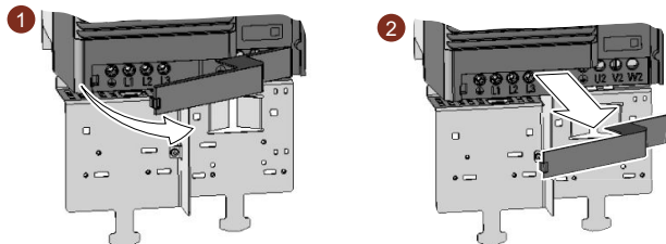
Figure 4-8 Removing the connection cover, FSD/FSE
