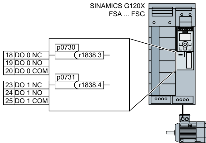
Figure 6-29 Feedback signal "STO is active" via digital outputs
