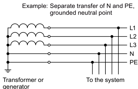
Figure 4-1 TN system
