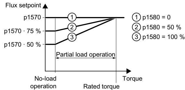
Figure 6-95 Reduce the flux setpoint in the partial load range of the motor
