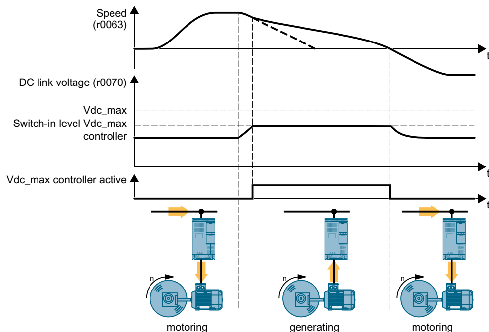
Figure 6-85 Simplified representation of the V_{dc\_max} control
