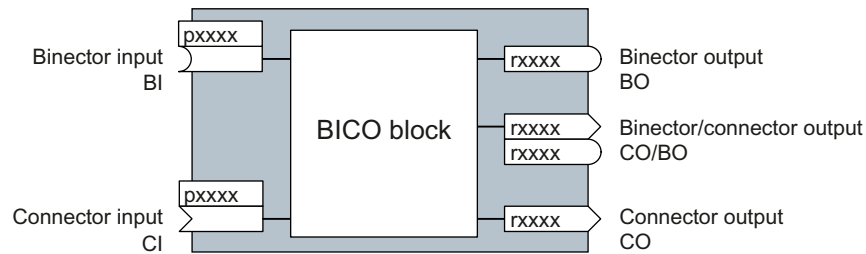
Figure 6-114 Symbols for binector and connector inputs and outputs
