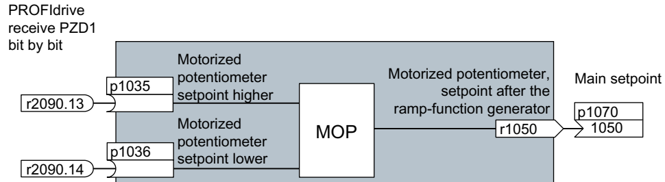
Figure 6-113 Example: Signal interconnection of two blocks for digital input 0
