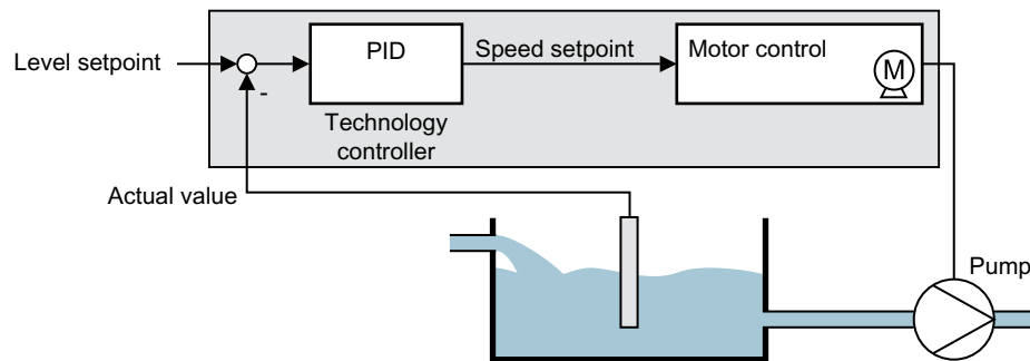
Figure 6-52 Example: Technology controller as a level controller
