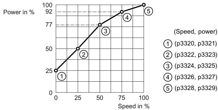
Figure 6-108 Factory setting of the flow characteristic
