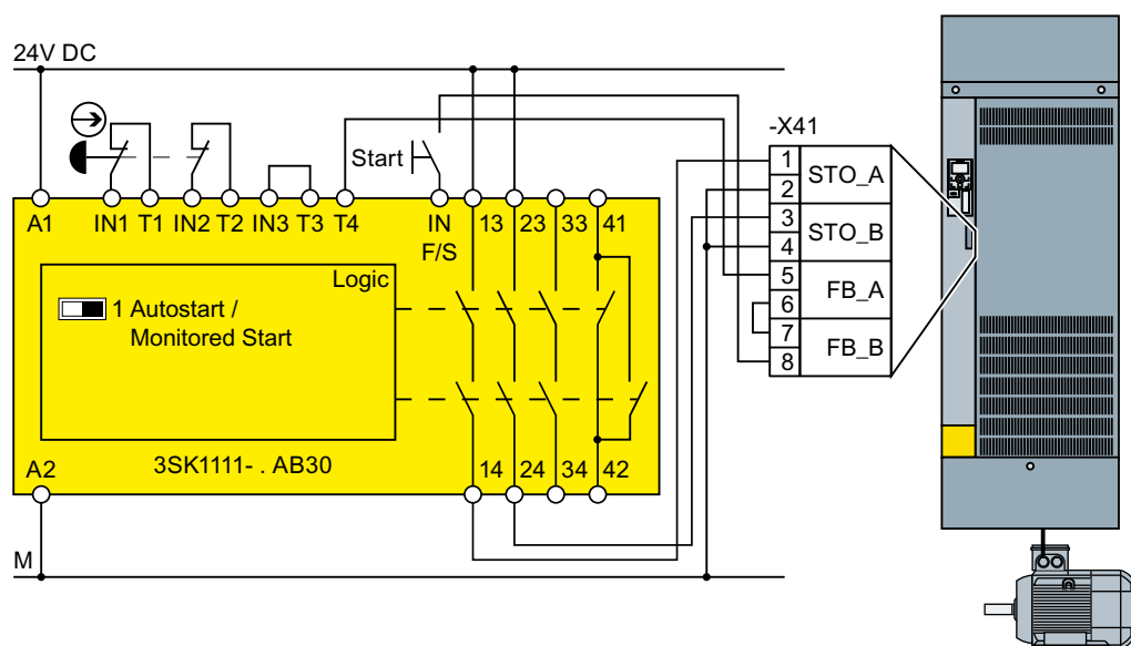
Figure 4-28 Connection 3SK1 inside a control cabinet for FSH, FSJ
