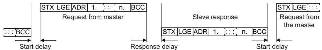
Figure 6-22 Start delay and response delay
