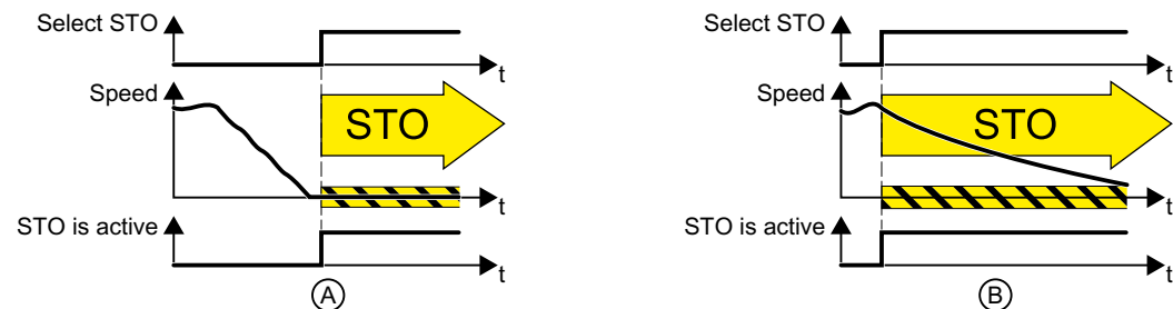
Figure 6-28 Functionality of STO when the motor is at standstill (A) and rotating (B)
