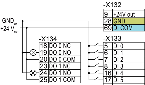
Figure 4-15 Connecting contacts switching to m potential with an external power supply
