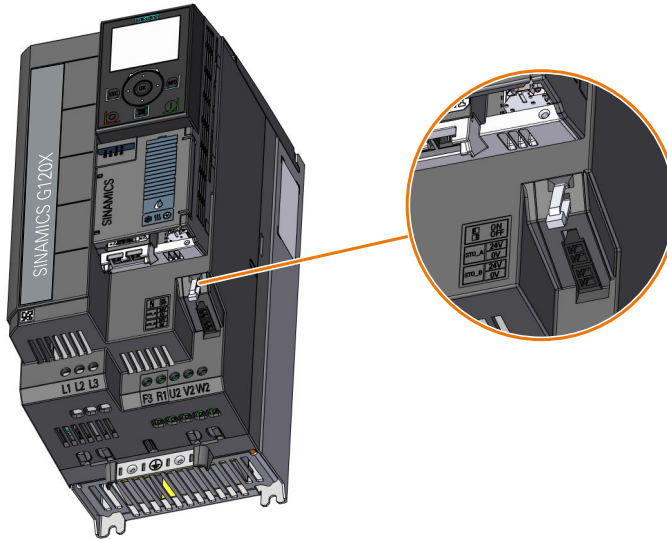
Figure 4-26 Protection against inadvertent inhibition of the "STO" function, FSA ... FSC
