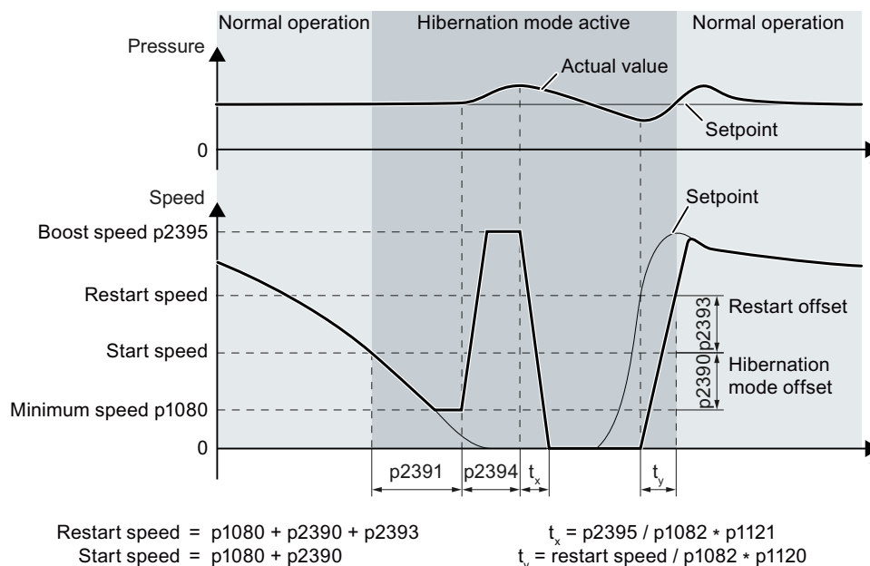
Figure 6-102 Hibernation mode using an external setpoint with boost
