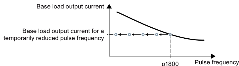
Figure 6-81 Derating characteristic and base load output current for overload
