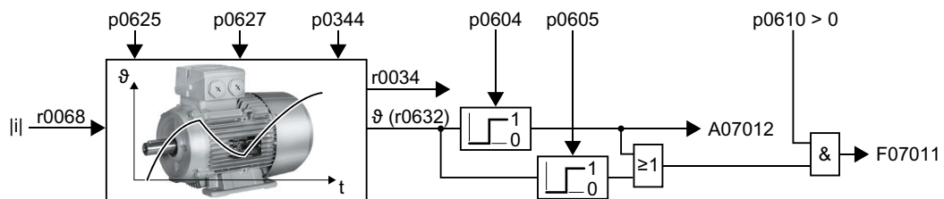
Figure 6-83 Thermal motor model 2 for induction motors
