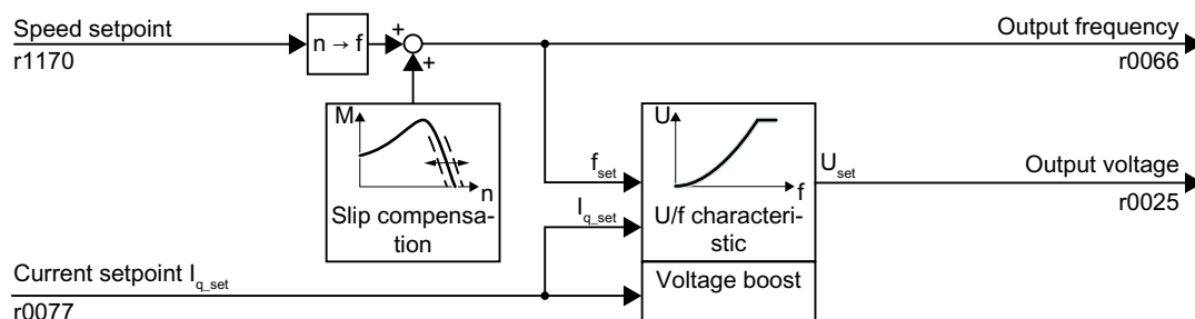
Figure 6-73 Default setting of the U/f control after selecting Standard Drive Control
