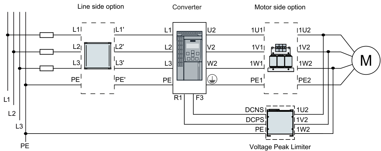
Figure 4-5 Connecting converters FSA ... FSG and their optional components
