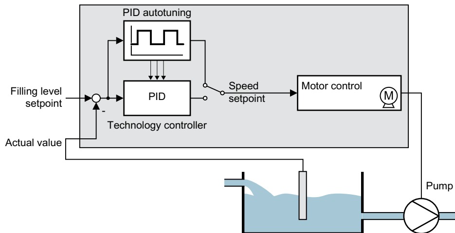
Figure 6-58 Autotuning using closed-loop level control as example
