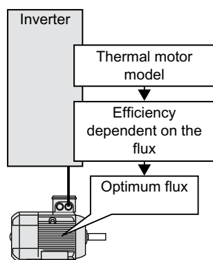
Figure 6-93 Determining the optimum flux from the motor thermal model
