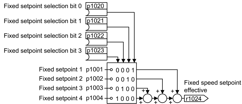
Figure 6-45 Direct selection of the fixed speed setpoint
