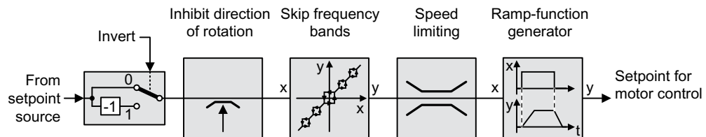
Figure 6-49 Setpoint processing in the converter
