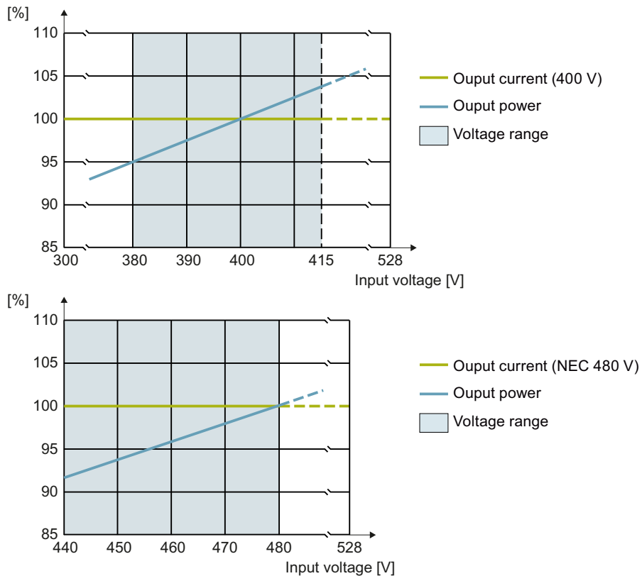
Figure 11-1 Current derating as a function of the input voltage for FSA ... FSG
