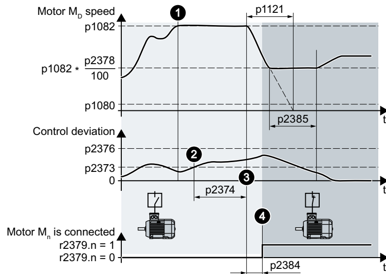
Figure 6-64 Activate uncontrolled motors M_1 \dots M_2
