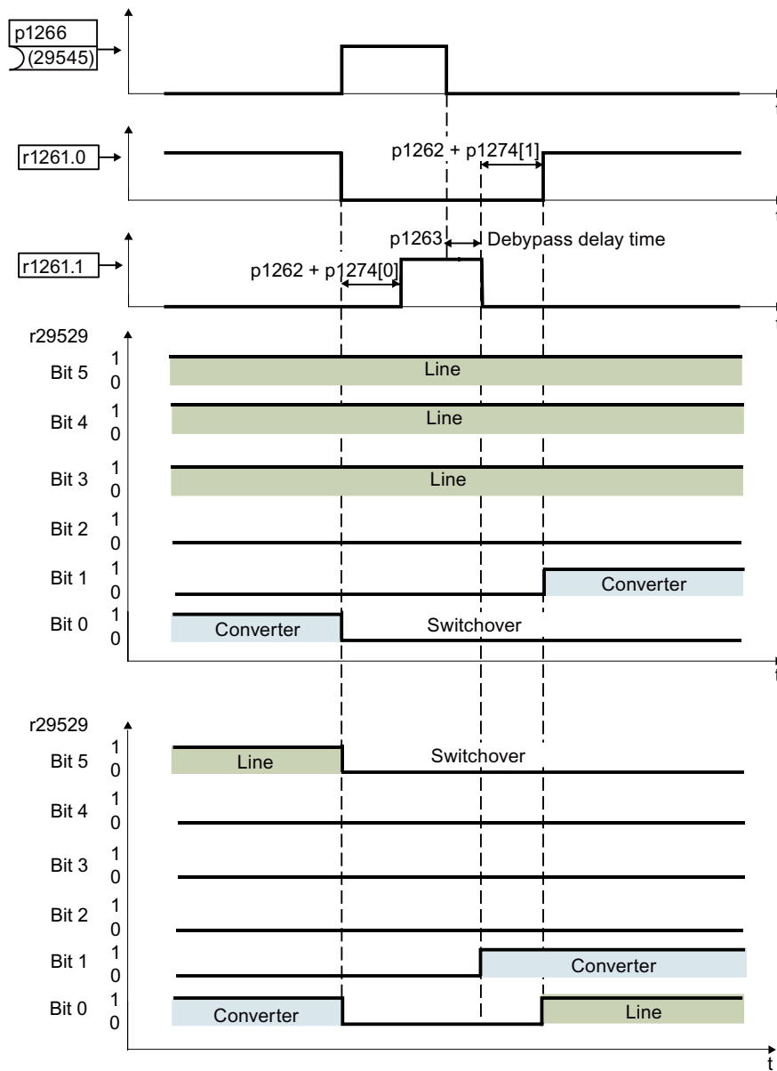
Figure 6-36 Pump switchover
