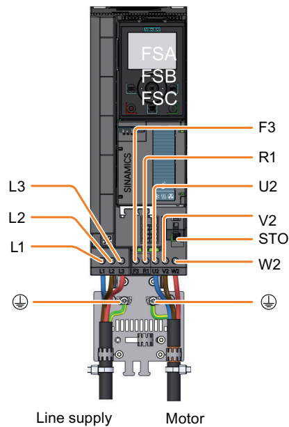
Figure 4-7 Connections for the line supply, motor and DC link terminals
