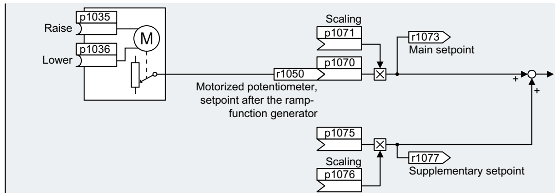
Figure 6-41 Motorized potentiometer as setpoint source
