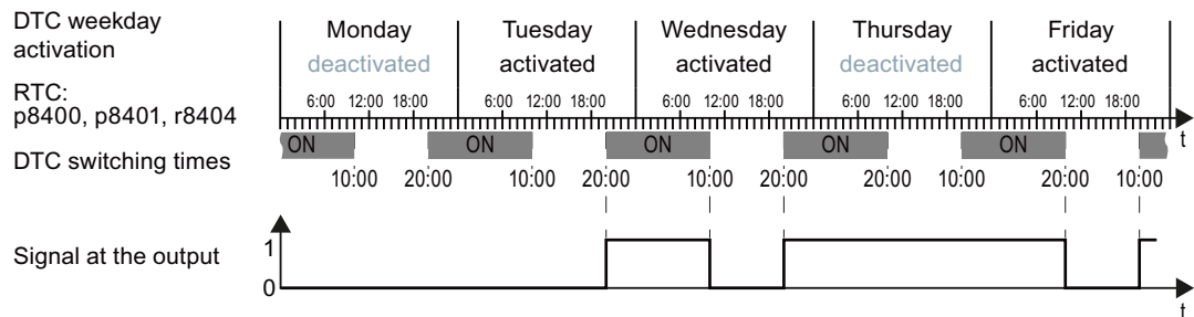
Figure 6-66 Example of the response of the time switch.
