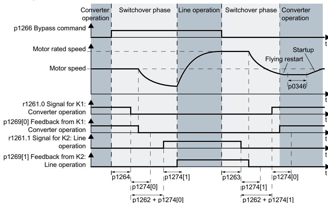
Figure 6-98 Changeover when activating via a control signal ( p1267.0 = 1 )
