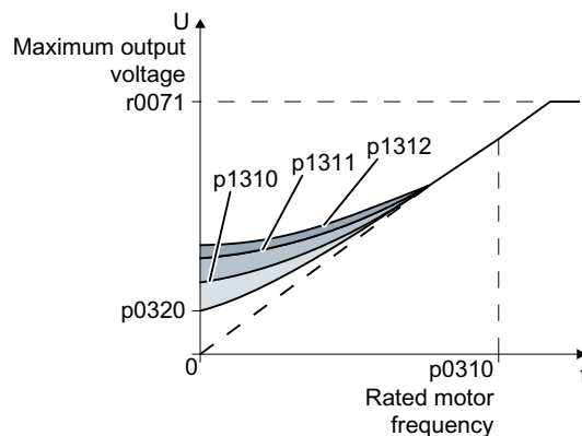
Figure 6-75 The resulting voltage boost using a linear characteristic as example
