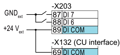
Figure 4-17 Connecting M-switching contacts
