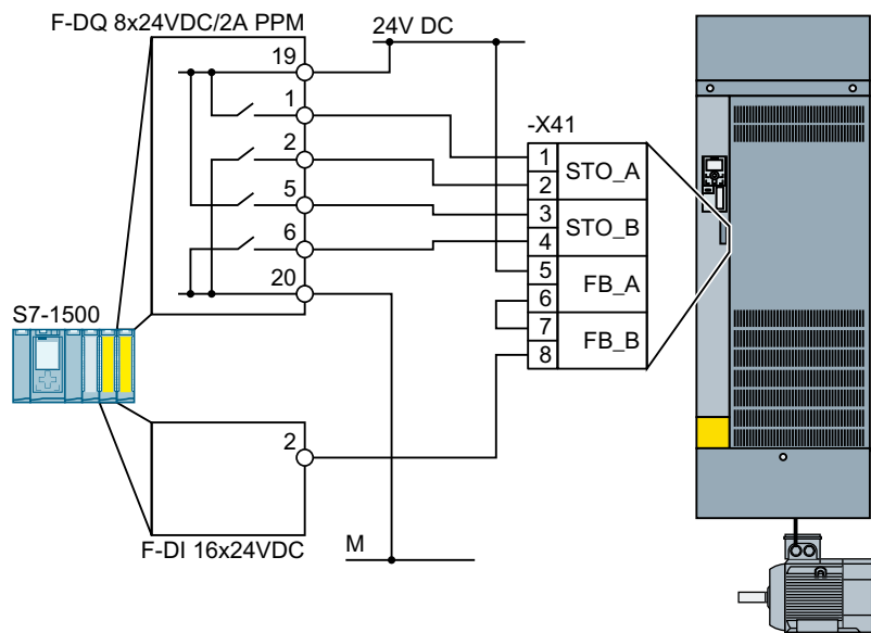
Figure 4-37 Connection of the SIMATIC S7-1500 inside a control cabinet for FSH and FSJ
