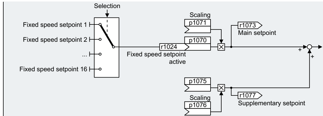
Figure 6-44 Fixed speed setpoint as setpoint source
