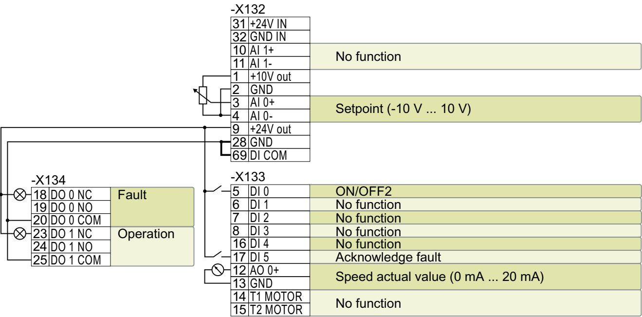
Figure 4-19 Factory setting for converters with RS 485 fieldbus interfaces
