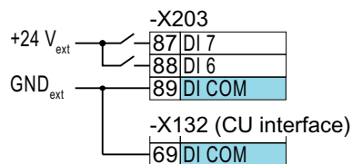
Figure 4-16 Connecting P-switching contacts
