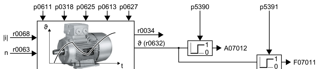
Figure 6-84 Thermal motor model 1 for reluctance motors
