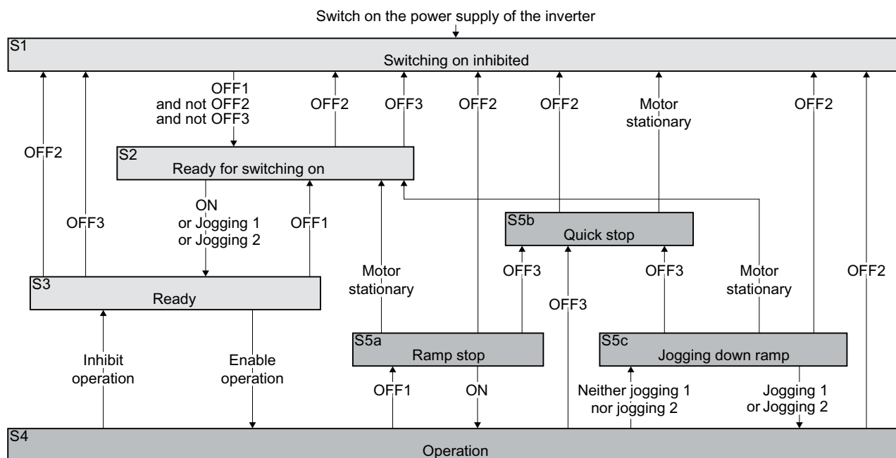
Figure 6-3 Sequence control of the converter when the motor is switched on and off
