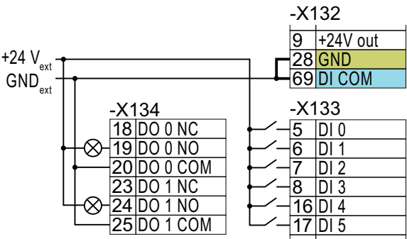
Figure 4-14 Connecting contacts switching to p potential with an external power supply
