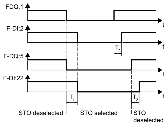
Figure 4-36 Dynamic monitoring of STO feedback for FSA ... FSG
