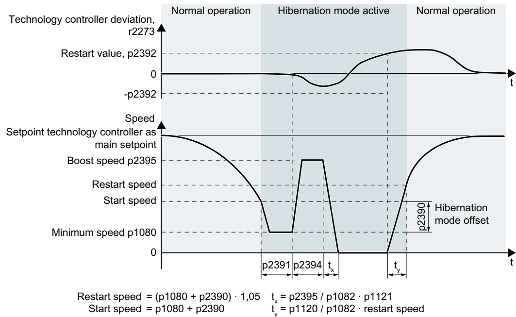
Figure 6-101 Hibernation mode using the technology setpoint as main setpoint with boost
