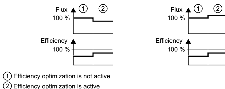
Figure 6-94 Qualitative result of efficiency optimization, method 2
