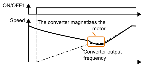
Figure 6-87 Principle of operation of the "flying restart" function
