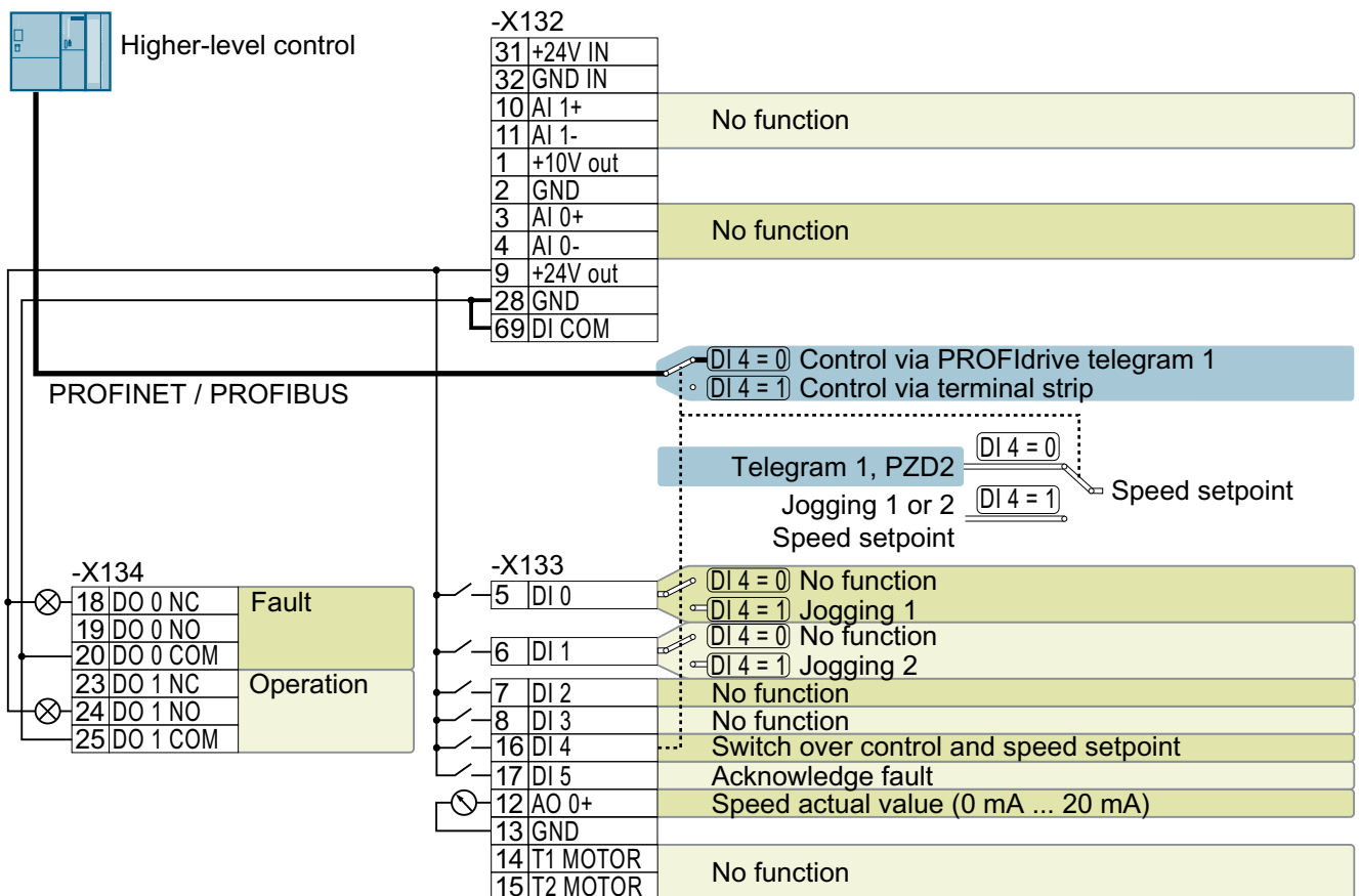
Figure 4-18 Factory setting for converters with PROFINET or PROFIBUS interfaces
