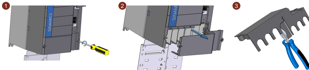
Figure 4-9 Removing the connection cover and making openings, FSF/FSG
