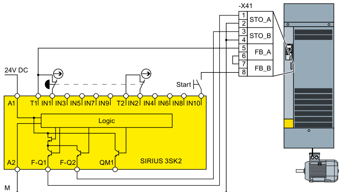
Figure 4-31 Connection 3SK2 inside a control cabinet for FSH and FSJ
