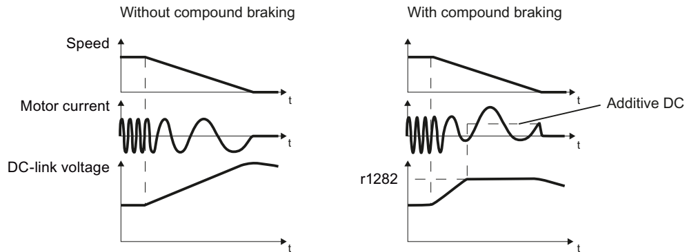
Figure 6-80 Motor brakes with and without active compound braking
