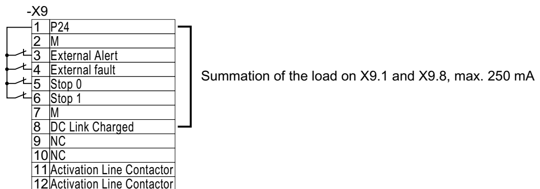
Figure 4-22 Terminal strip X9 with internal 24 V supply
