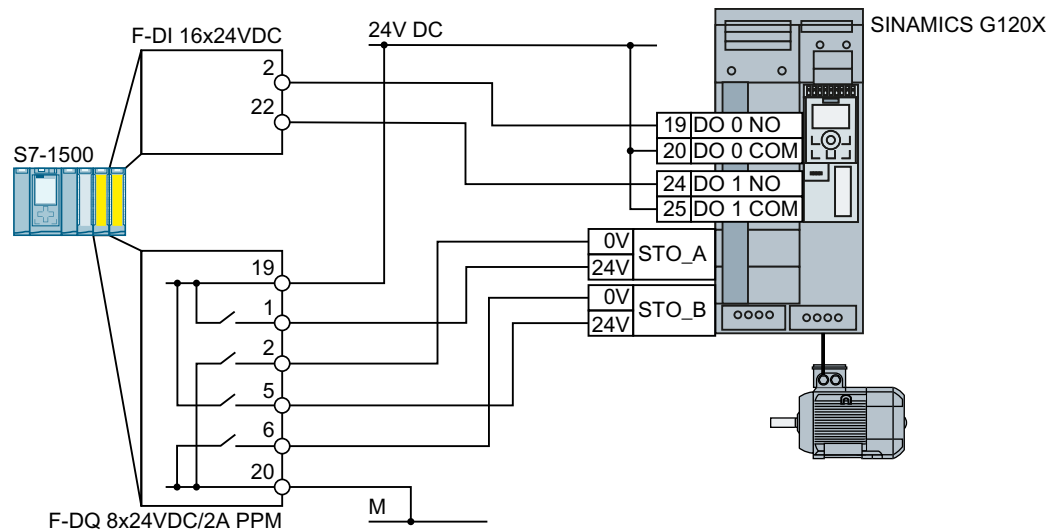
Figure 4-35 Connecting the SIMATIC S7-1500 in a control cabinet for FSA ... FSG
