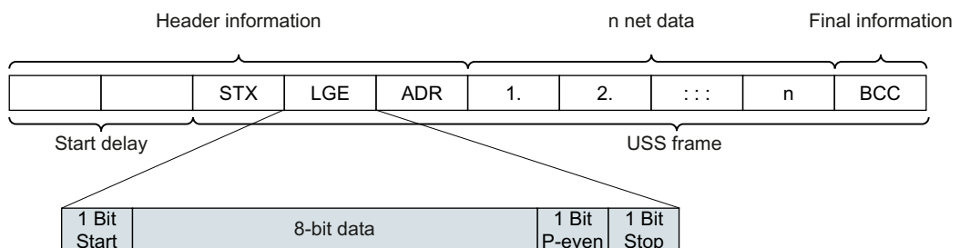
Figure 6-18 Structure of a USS telegram
