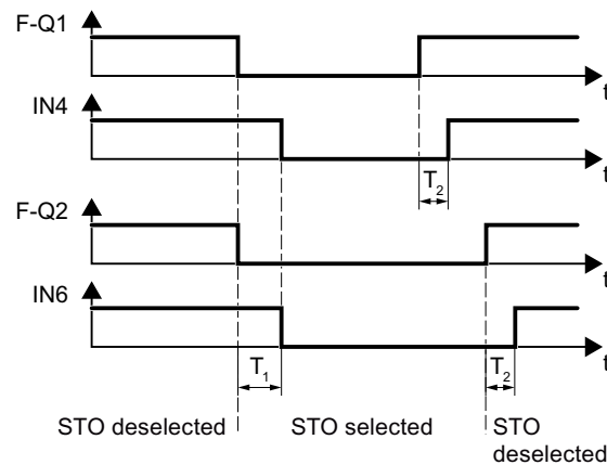
Figure 4-30 Dynamic monitoring of STO feedback for FSA ... FSG
