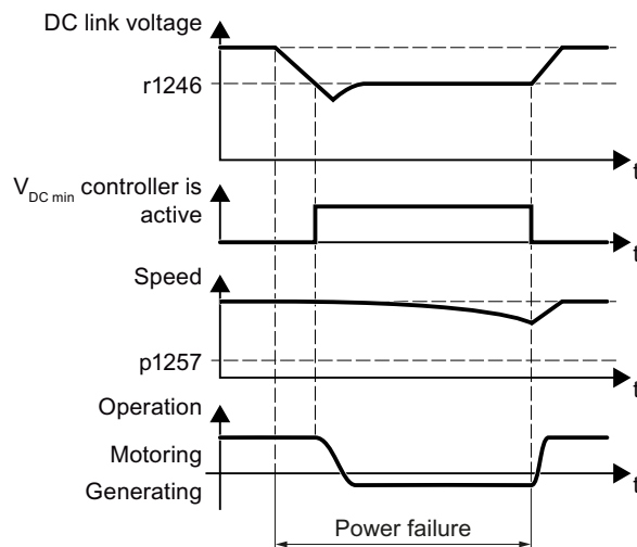
Figure 6-90 Principle mode of operation of kinetic buffering
