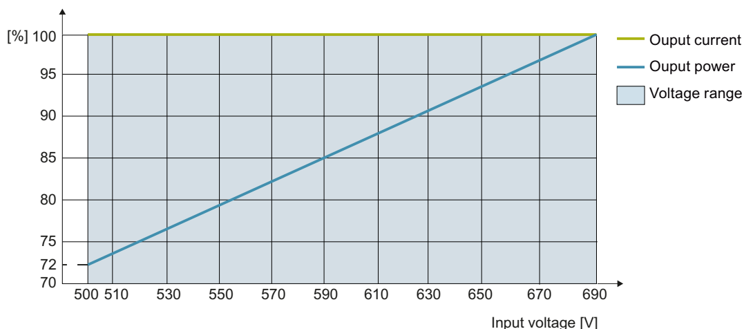
Figure 11-3 Current derating as a function of the input voltage for FSA ... FSG
