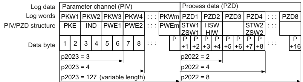
Figure 6-19 USS telegram - user data structure
