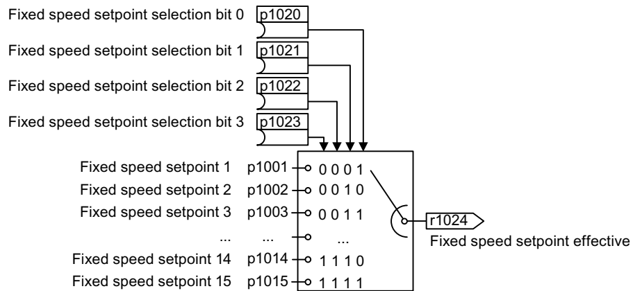
Figure 6-46 Binary selection of the fixed speed setpoint
