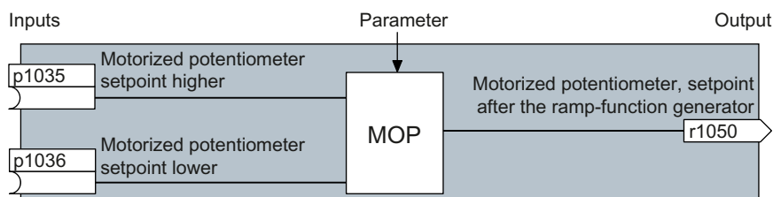
Figure 6-112 Example of a block: Motorized potentiometer (MOP)
