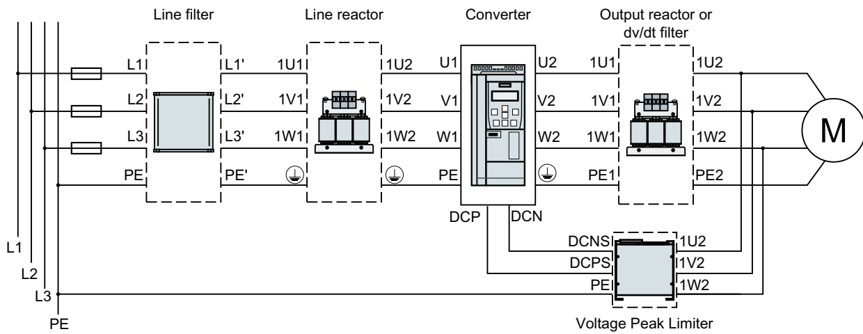
Figure 4-6 Connecting converters FSH/FSJ and their optional components
