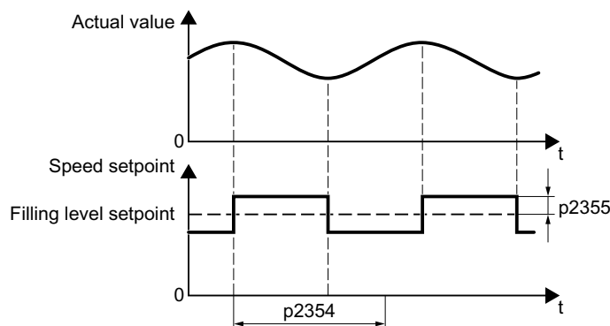
Figure 6-59 Example for speed setpoint and actual process value for autotuning
