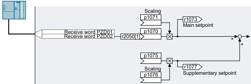
Figure 6-40 Fieldbus as setpoint source
