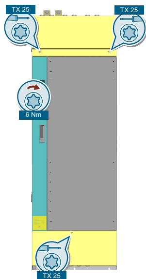
Figure 4-11 Removing the front cover
