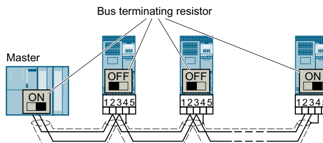
Figure 4-40 Connection with the fieldbus via RS485
