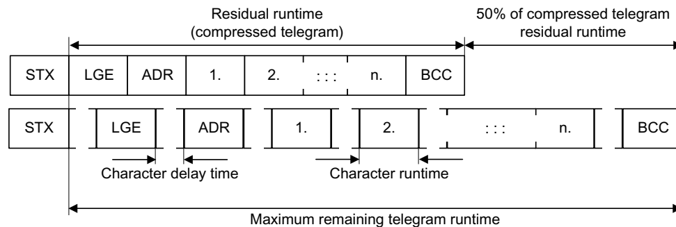
Figure 6-21 Telegram runtime as the sum of the residual runtime and character delay times
