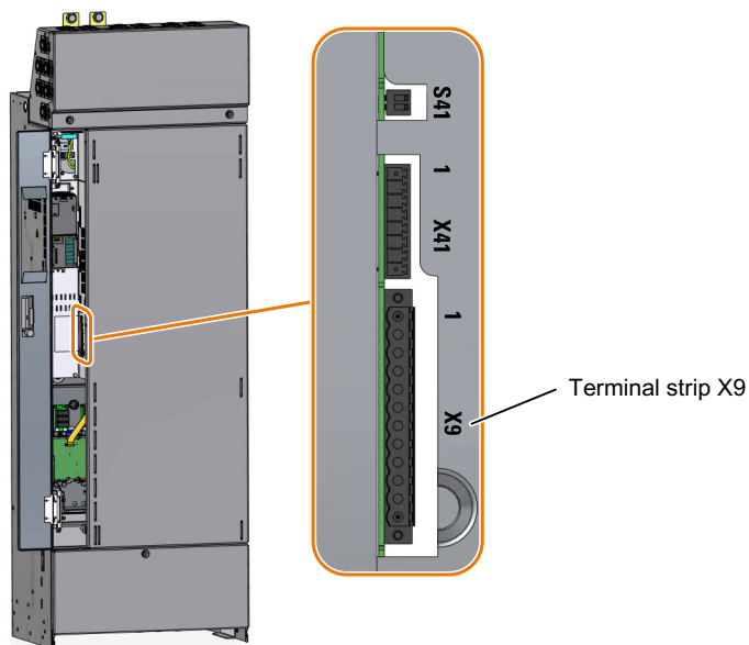
Figure 4-20 Terminal strip X9
