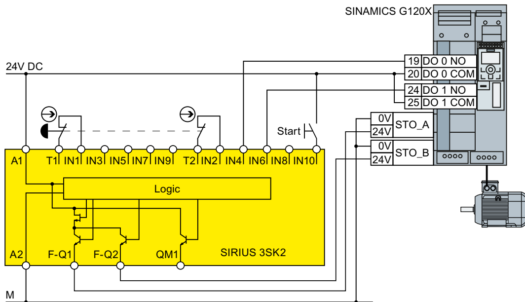
Figure 4-29 Connection 3SK2 inside a control cabinet for FSA ... FSG
