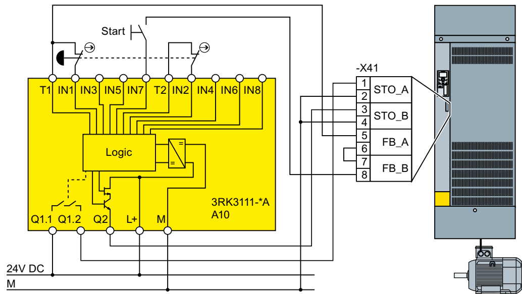
Figure 4-34 Connection 3RK3 inside a control cabinet for FSH and FSJ
