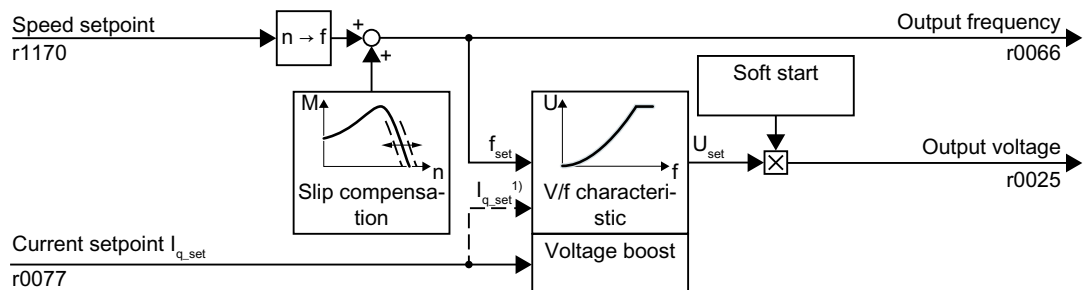
Figure 6-67 Simplified function diagram of the U/f control
