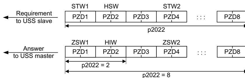
Figure 6-20 Process data channel
