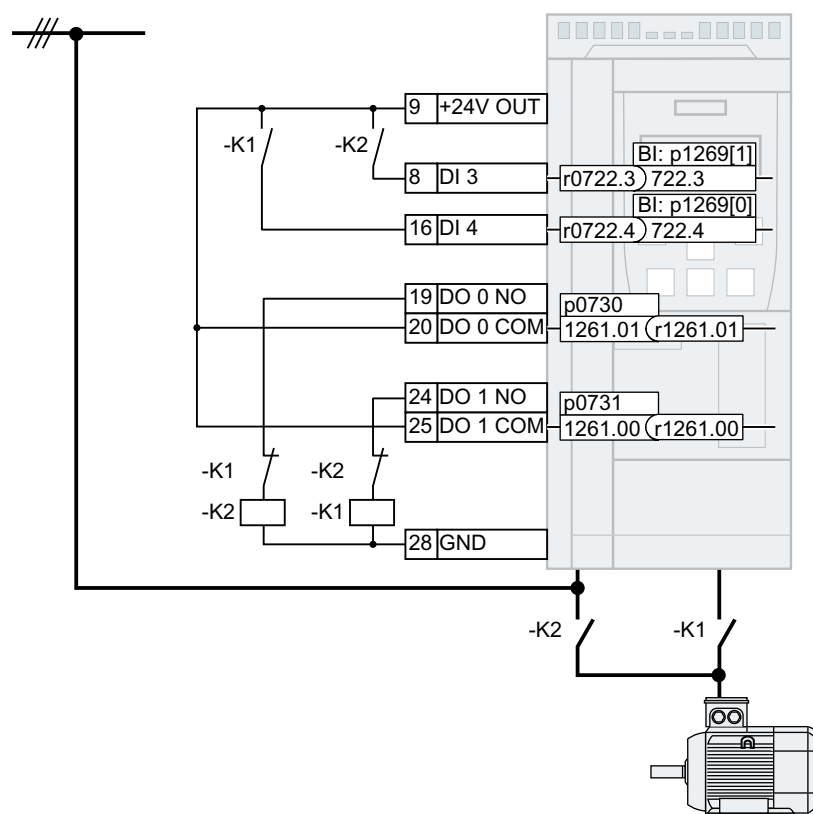
Figure 6-97 Bypass control via converter
