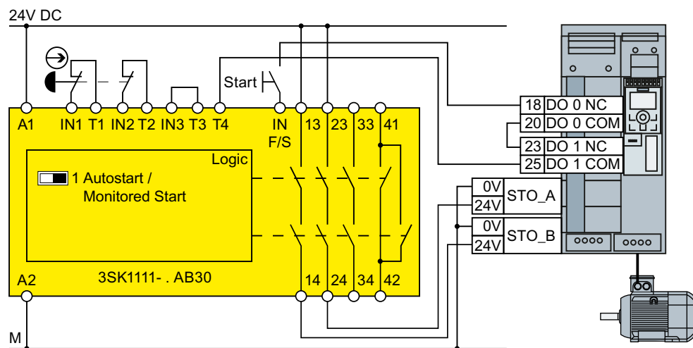
Figure 4-27 Connection 3SK1 inside a control cabinet for FSA ... FSG
