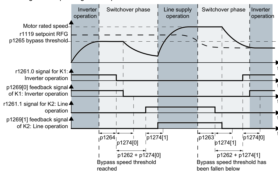
Figure 6-99 Changeover depending on the speed ( p1267.1 = 1 )
