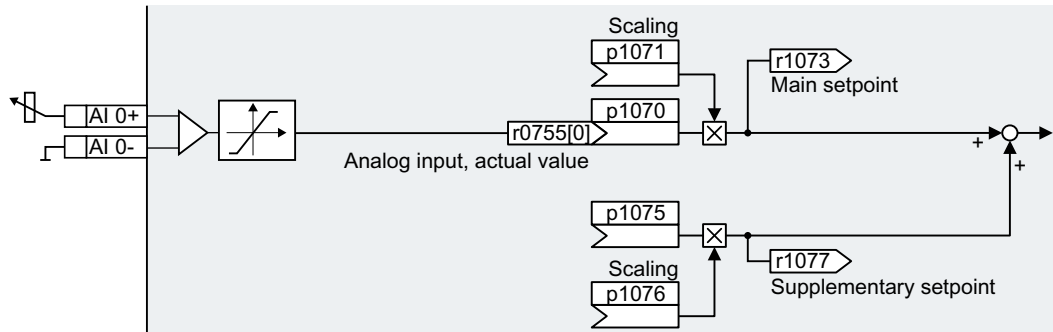
Figure 6-39 Example: Analog input 0 as setpoint source
