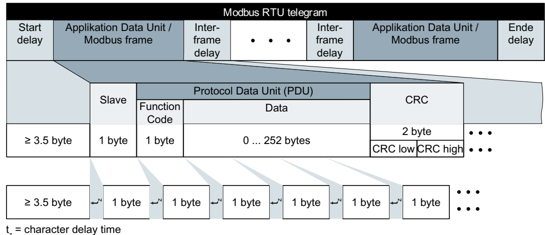
Figure 6-17 Modbus with delay times
