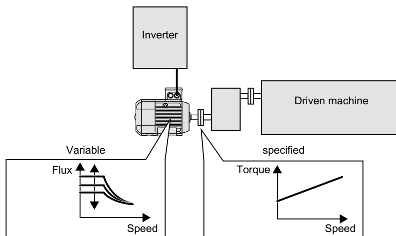
Figure 6-92 Efficiency optimization by changing the motor flux
