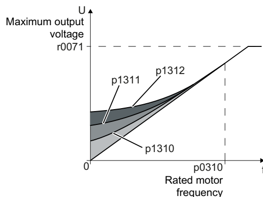
Figure 6-70 The resulting voltage boost using a linear characteristic as example
