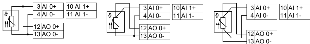
Figure 6-82 Two-wire connection, three-wire connection and four-wire connection
