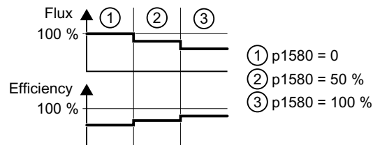
Figure 6-96 Qualitative result of efficiency optimization, method 1
