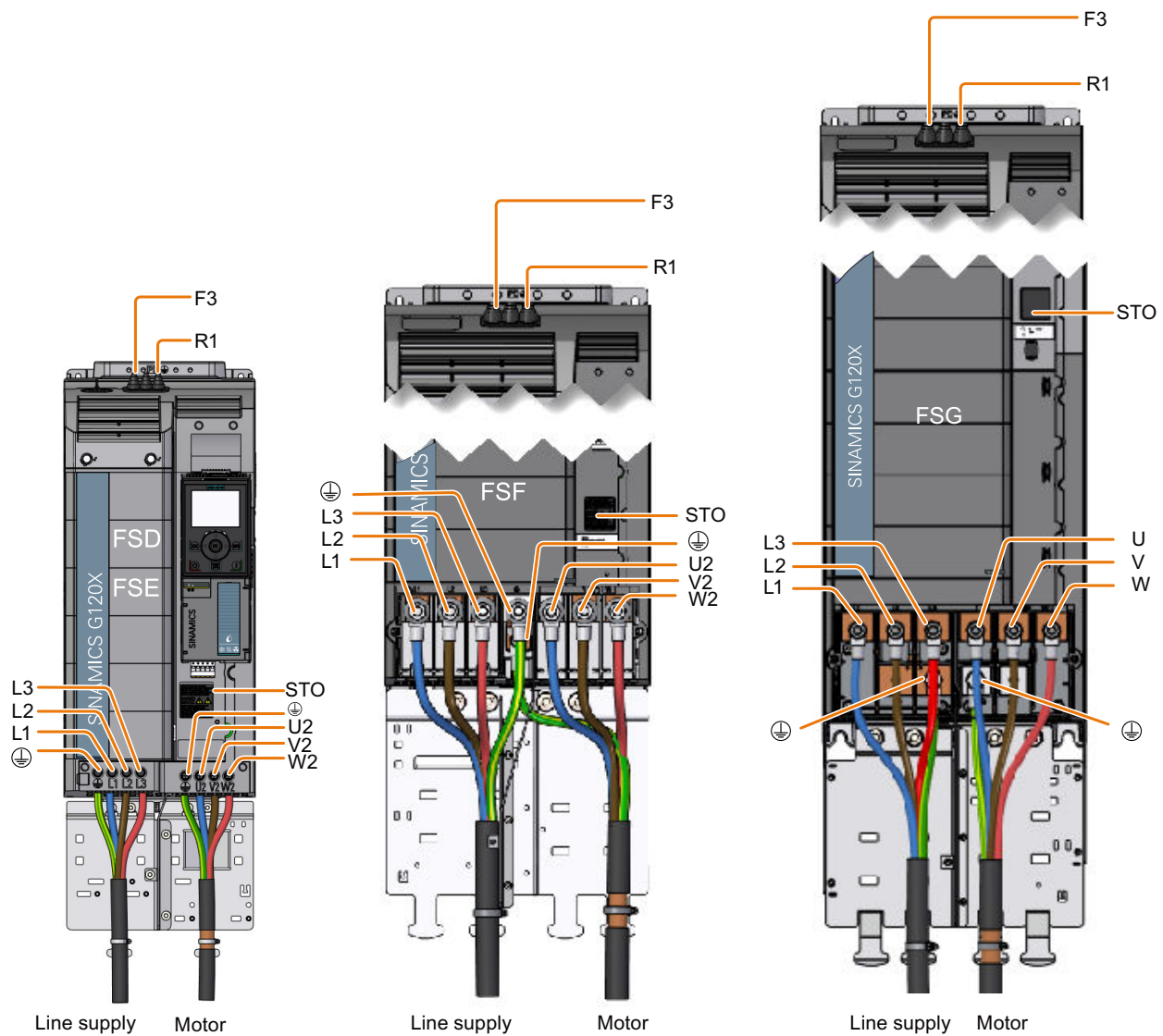
Figure 4-10 Connections for the line supply and motor
