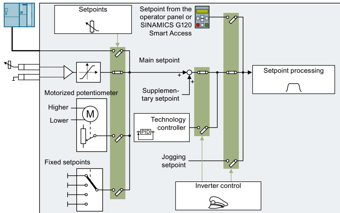
Figure 6-38 Setpoint sources for the converter
