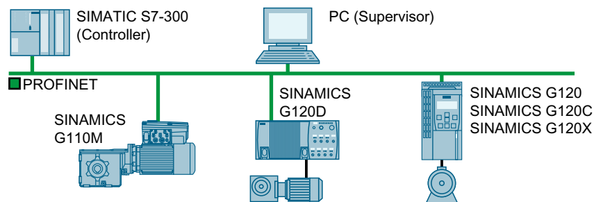
Figure 4-38 The converter in PROFINET IO operation
