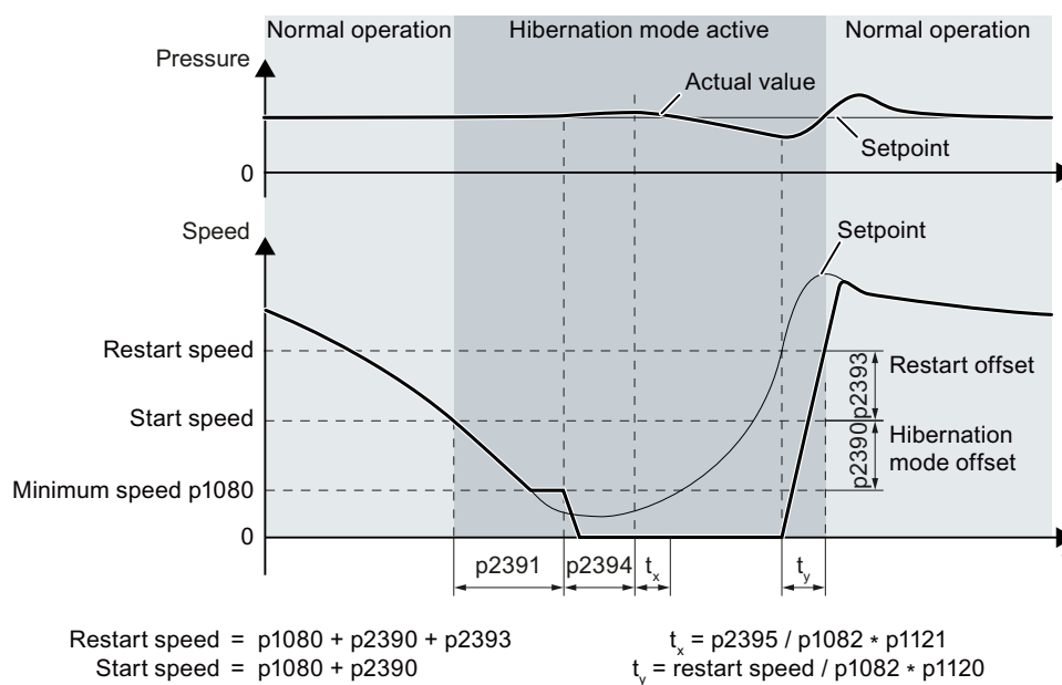
Figure 6-103 Hibernation mode using an external setpoint without boost
