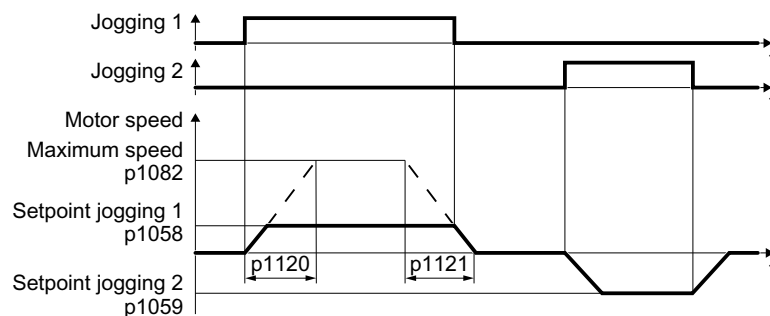
Figure 6-27 Behavior of the motor when "jogging"
