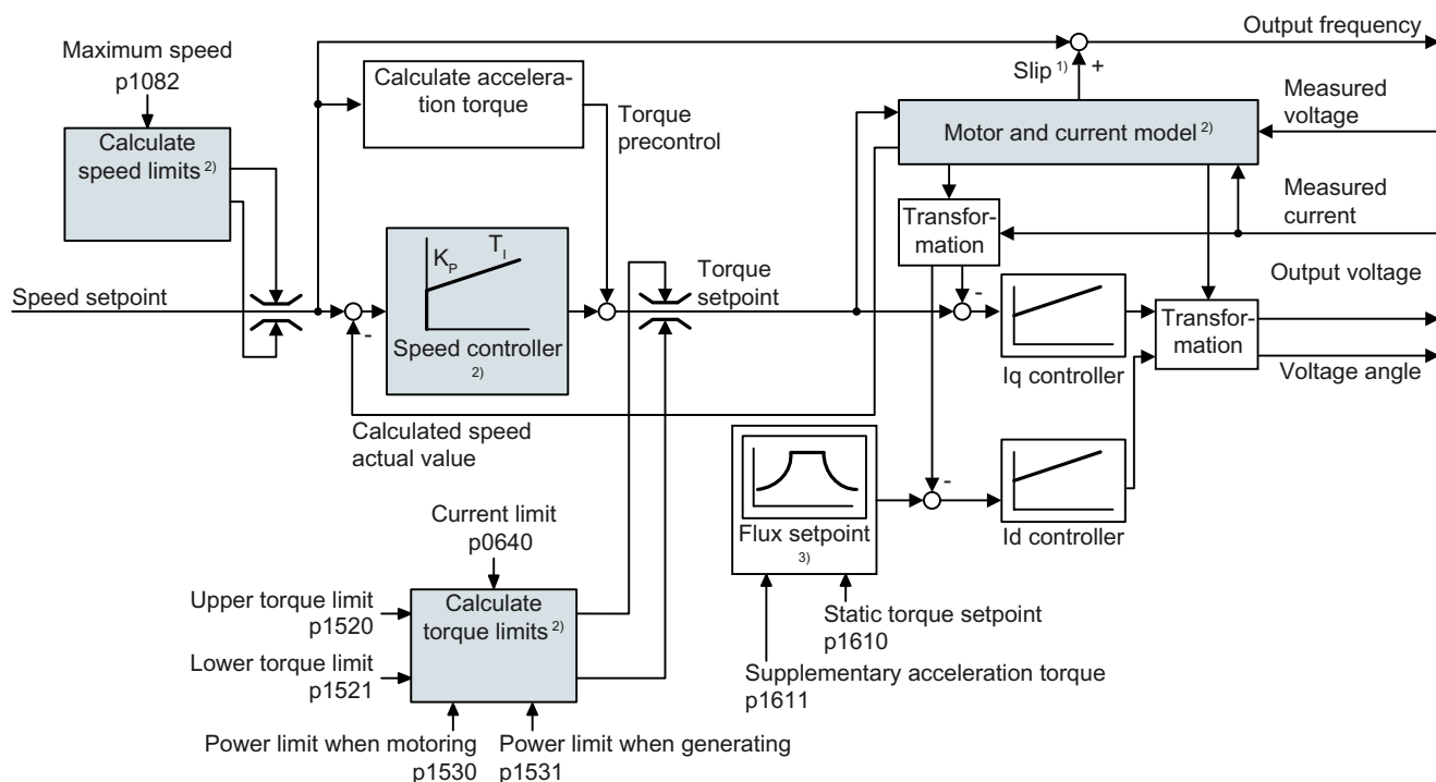
Figure 6-76 Simplified function diagram for sensorless vector control with speed controller
