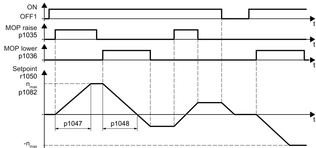
Figure 6-42 Function chart of the motorized potentiometer
