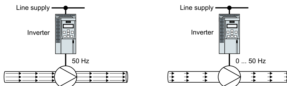
Figure 6-107 Flow control with pump and converter
