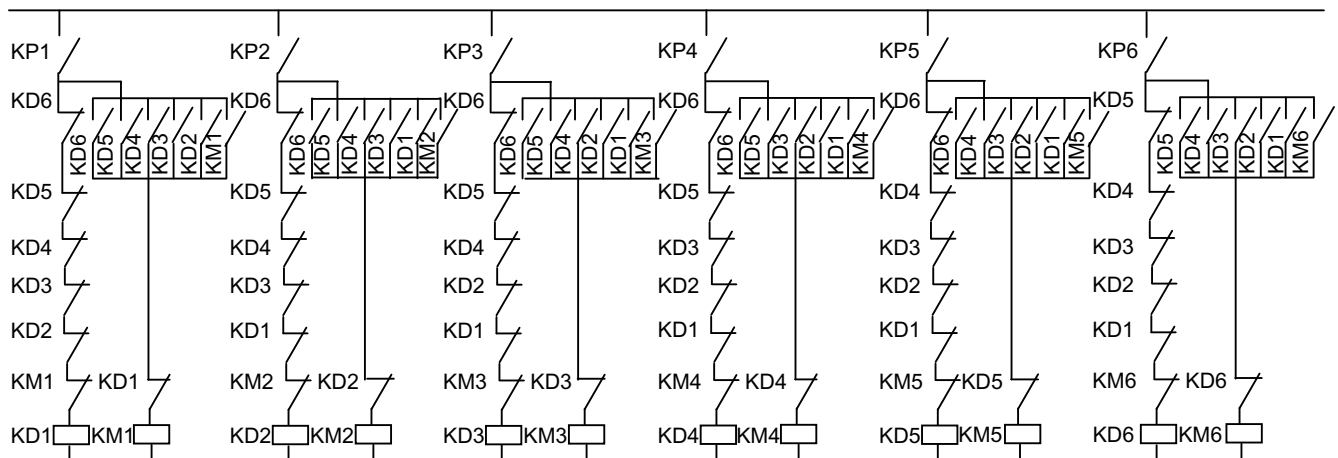
Figure 6-31 External relay control circuit
