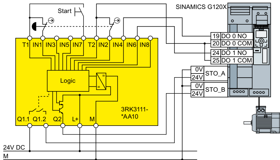
Figure 4-32 Connection 3RK3 inside a control cabinet for FSA ... FSG
