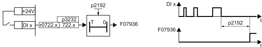
Figure 6-86 Function plan and time response of the speed monitoring
