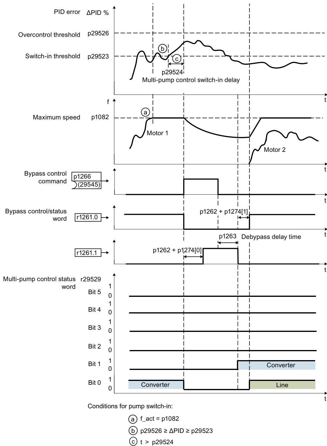
Figure 6-32 Pump switch-in
