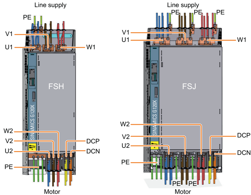
Figure 4-12 Connections for the line supply, motor and DC link terminals
