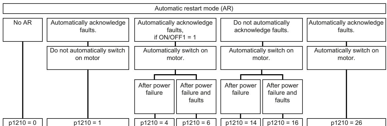
Figure 6-88 Automatic restart modes
