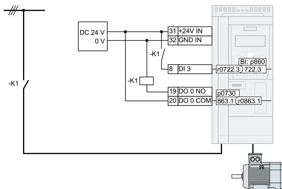
Figure 6-104 Line contactor control via DO 0 with feedback signal via DI 3
