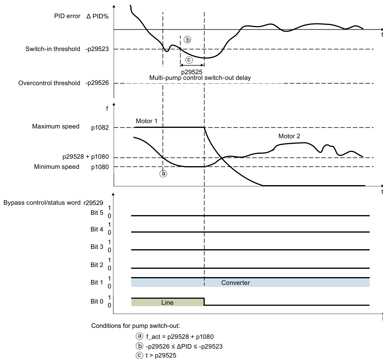
Figure 6-34 Pump switch-out based on the absolute operating hours (p29522 = 1)
