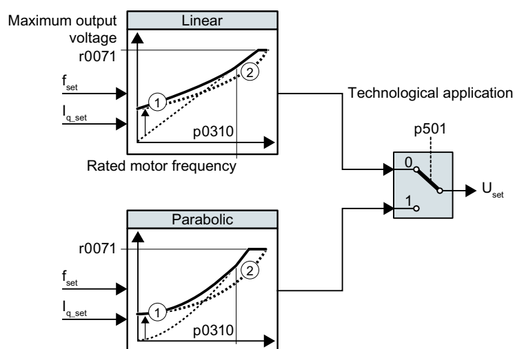
Figure 6-74 Characteristics after selecting Standard Drive Control
